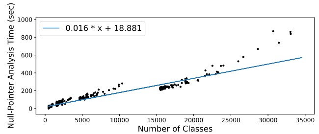
Figure 15: Class-budget and analysis time relationship.
