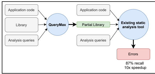
Figure 1: Overview of the QueryMax workflow
